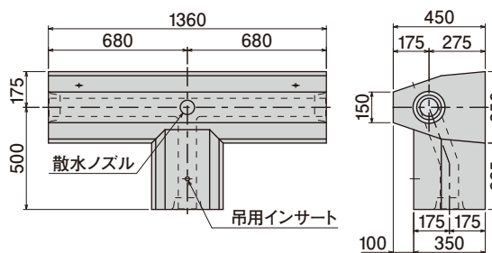
偏心T型E100
