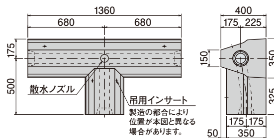
偏心T型E50
